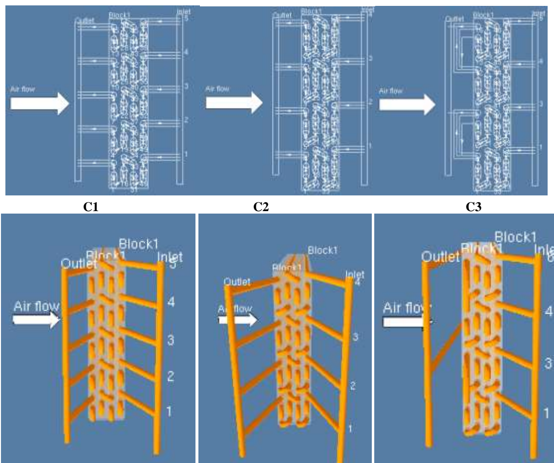
Figure 4: Circuit designs (top) and simulation results (bottom) of C-Series of 5 mm condenser.
