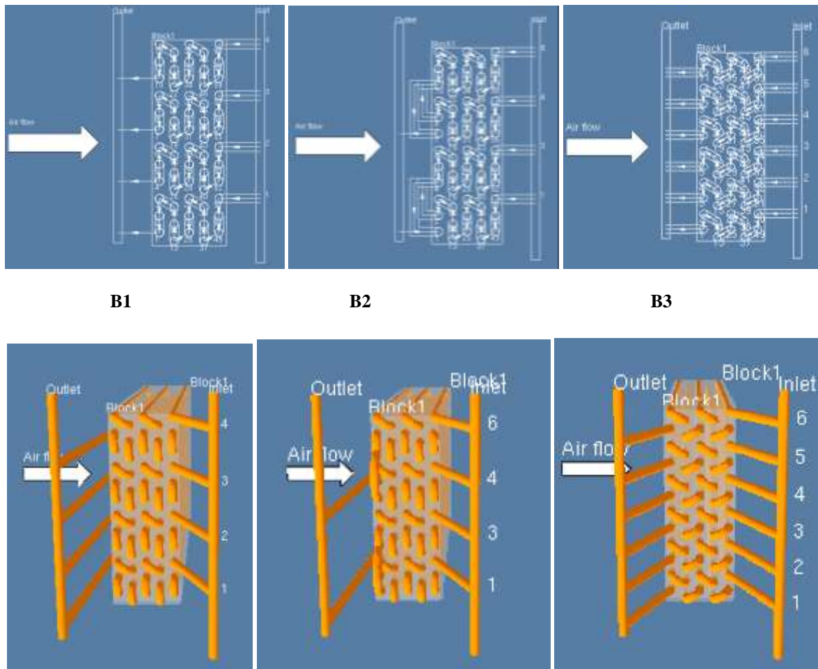
Figure 3: Circuit designs (top) and simulation results (bottom) of B-Series of 5 mm condenser with 60 tubes.
