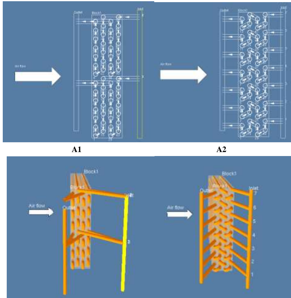
Figure 2: Circuit designs (top) and simulation results (bottom) of A-Series of 5 mm condenser with 52 tubes.
